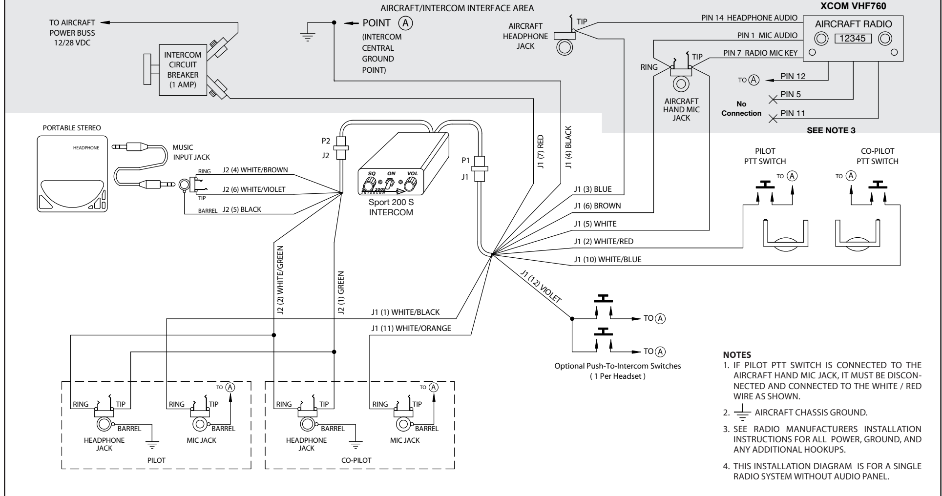
Sport 200S – XCOM VHF760 Radio Installation Wiring Diagram
