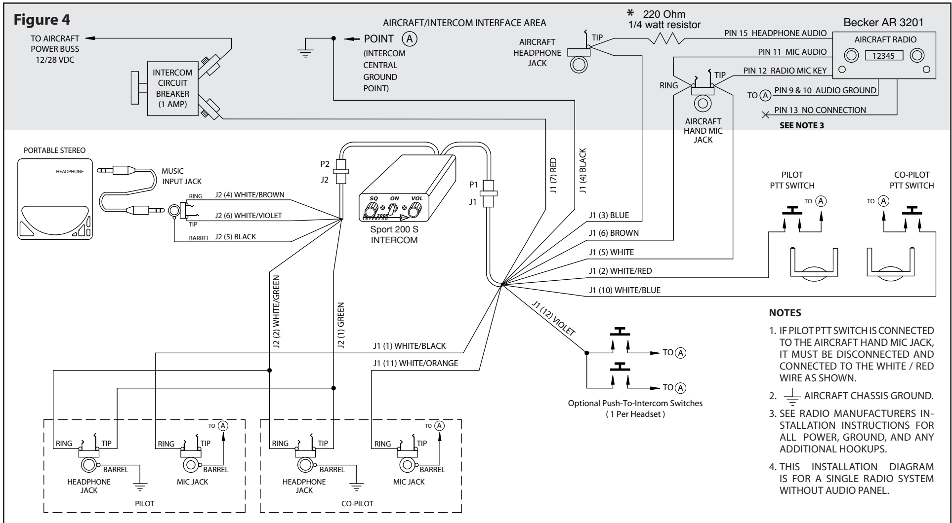
Sport 200S – Becker AR 3201 Radio Installation Wiring Diagram
